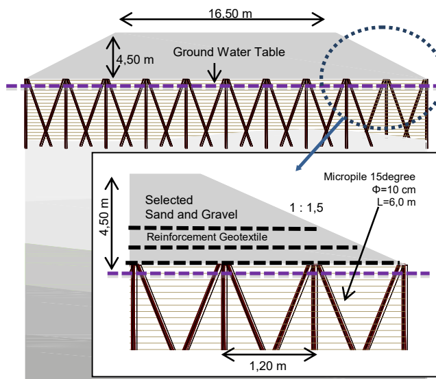
Figure 2a. Cross section of embankment
